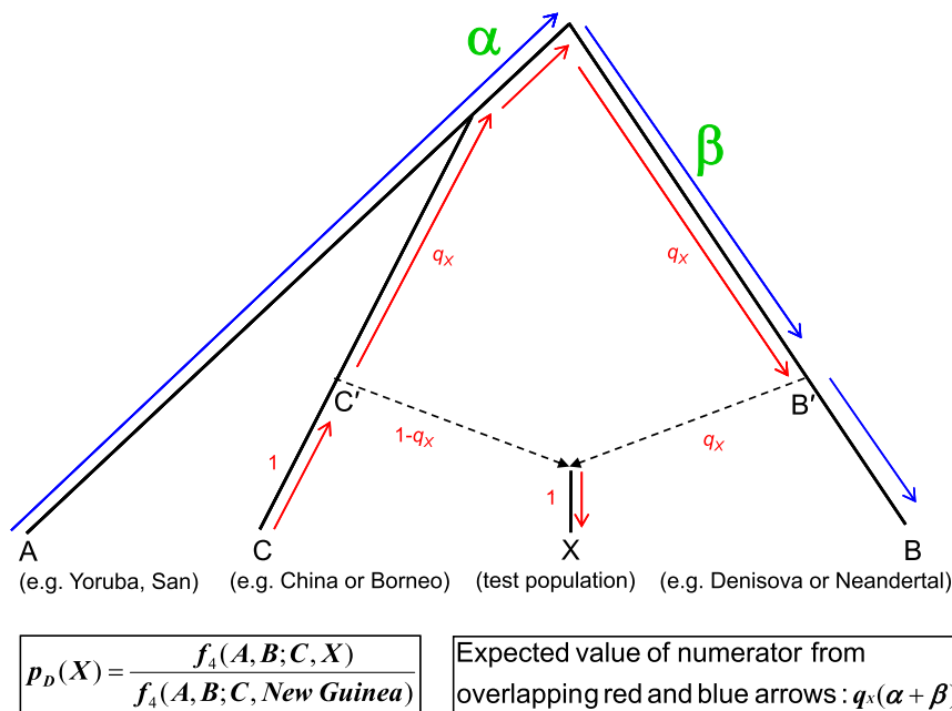
Figure 4. Computation of the Estimate of Denisovan Ancestry p_D(X)
