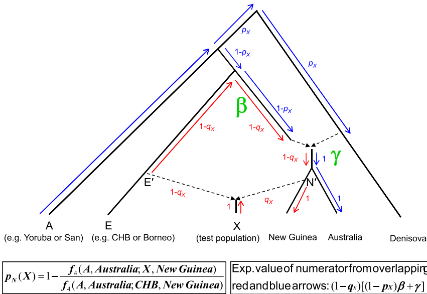
Figure 5. Computation of the Estimate of Near Oceanian Ancestry p_N(X)
