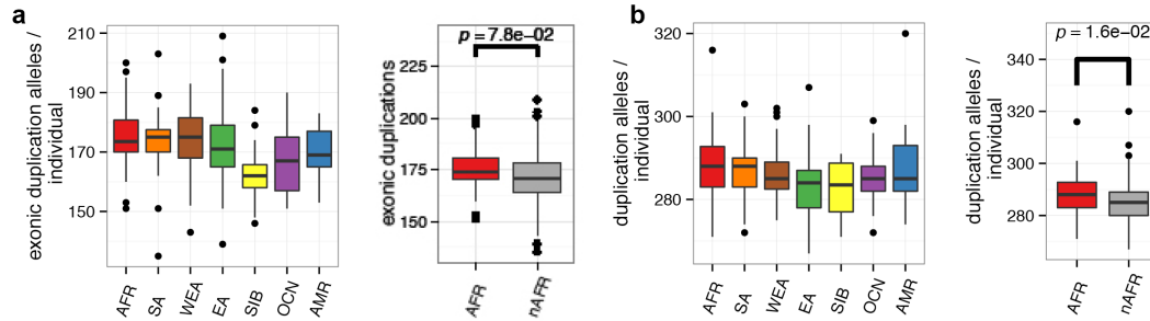
Figure S29: Boxplots of the number of exonic and intergenic duplication alleles per individual in different human populations are plotted in a and b, respectively, demonstrating no difference between African and non-African individuals.
