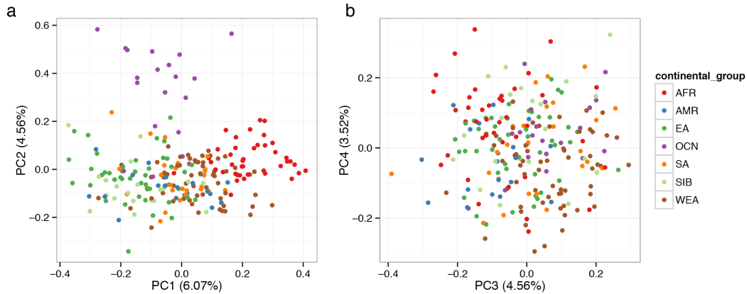
Figure S21: PCA of bi-allelic 2,3,4 duplication copy number state CNVs. PC1 and PC2 reconstruct the population structure of individuals, however, less clearly than deletions. PC3 and PC4 do not appear to distinguish population differences as was observed for deletions.
