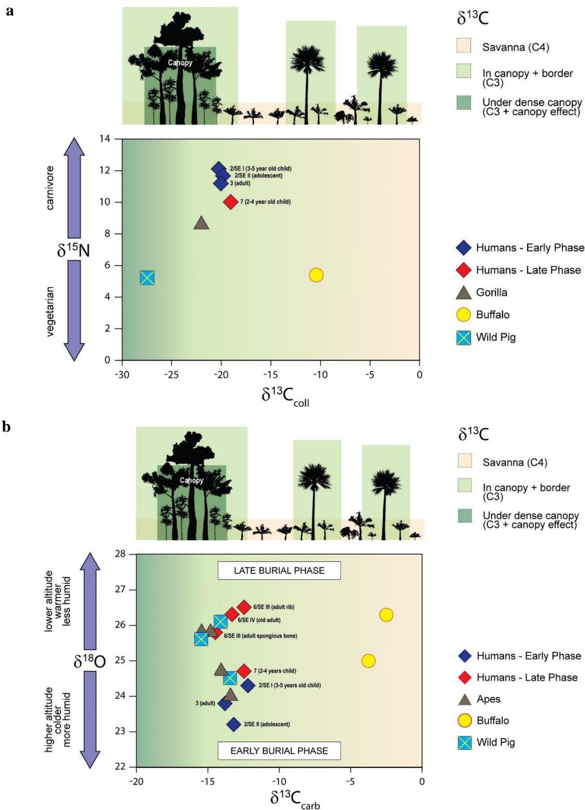
Figure S4: Preliminary results of the isotopic analyses from Shum Laka for human and faunal remains. Graph by H. Bocherens and modified by I. Ribot & O. Graf.
