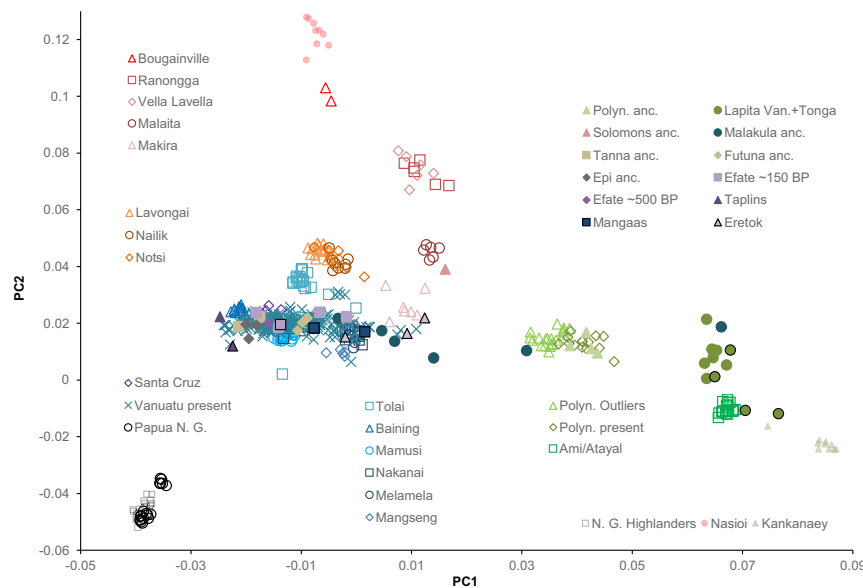
Figure 2. PCA Results
