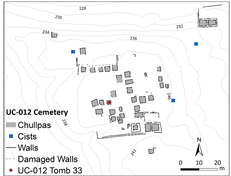
Figure S1. Site plans for the UC-008 and UC-012 cemeteries, showing the locations of UC-008 Tomb 1 and UC-012 Tomb 33.
