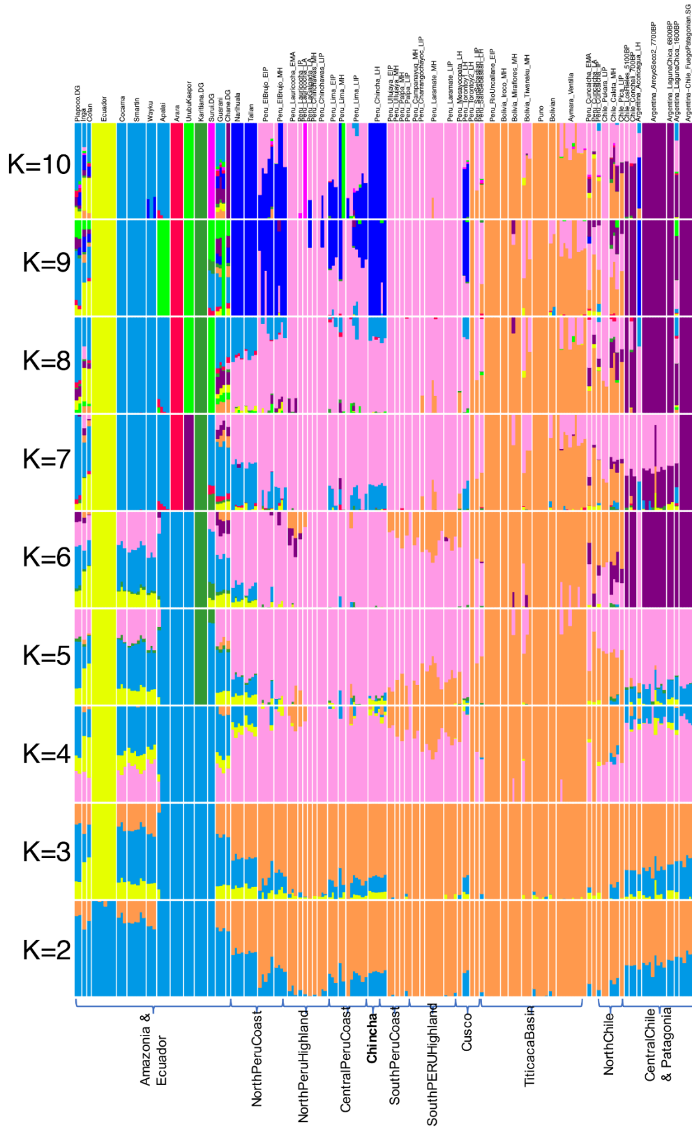
Figure S2. ADMIXTURE plot at different K values. The run with the highest log-likelihood score after 100 trials was taken for each K value.
